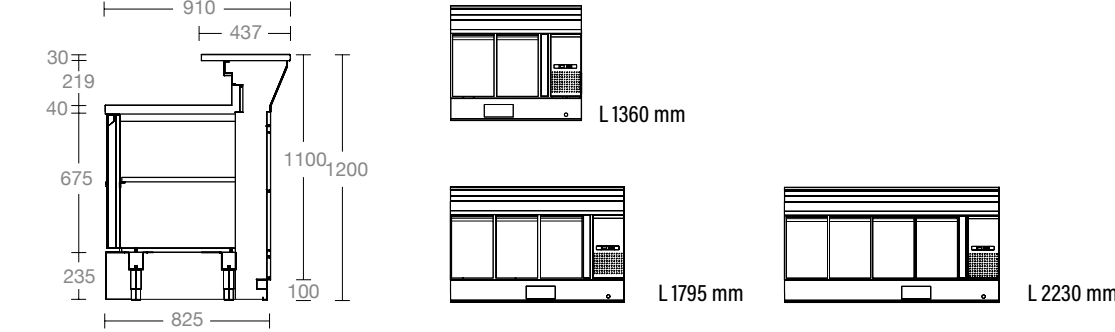
BANCO BAR CON CELLE REFRIGERATE VENTILATE E MOTORE INCORPORATO H1200 P825 MM BAR COUNTER WITH VENTILATED REFRIGERATED ROOMS & HERMETIC UNIT H1200 D825 MM
