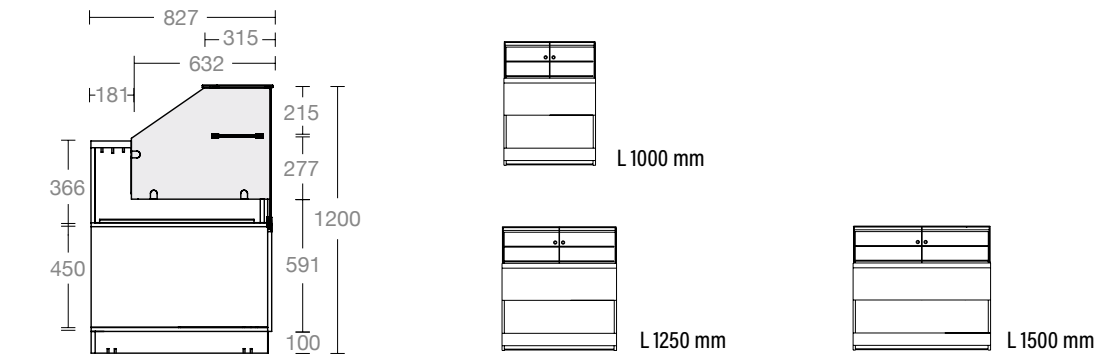
VETRINA PANETTERIA NEUTRO H1200 P825 MM BAKERY AMBIENT DISPLAY CASE H1200 D827 MM
