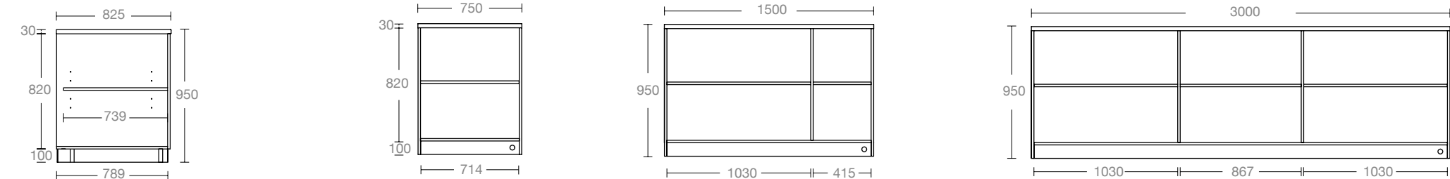
BANCO NEUTRO H950 P825 MM AMBIENT COUNTER H950 D825 MM BANCO NEUTRO L750 H950 P825 MM AMBIENT COUNTER W750 H950 D825 MM BANCO NEUTRO L1500 H950 P825 MM AMBIENT COUNTER W1500 H950 D825 MM BANCO NEUTRO L3000 H950 P825 MM AMBIENT COUNTER W3000 H950 D825 MM
