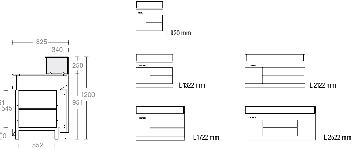
BANCO DROP-IN CALDO SECCO H1200 P825 mm HOT DRY DROP-IN COUNTER H1200 D825 MM
