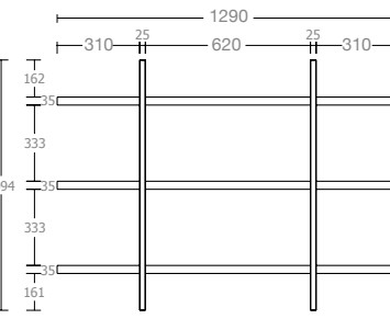
RETROALZATA BOTTIGLIERA BIMAT P 270 BIMAT BOTTLE COMPARTMENT D 270
